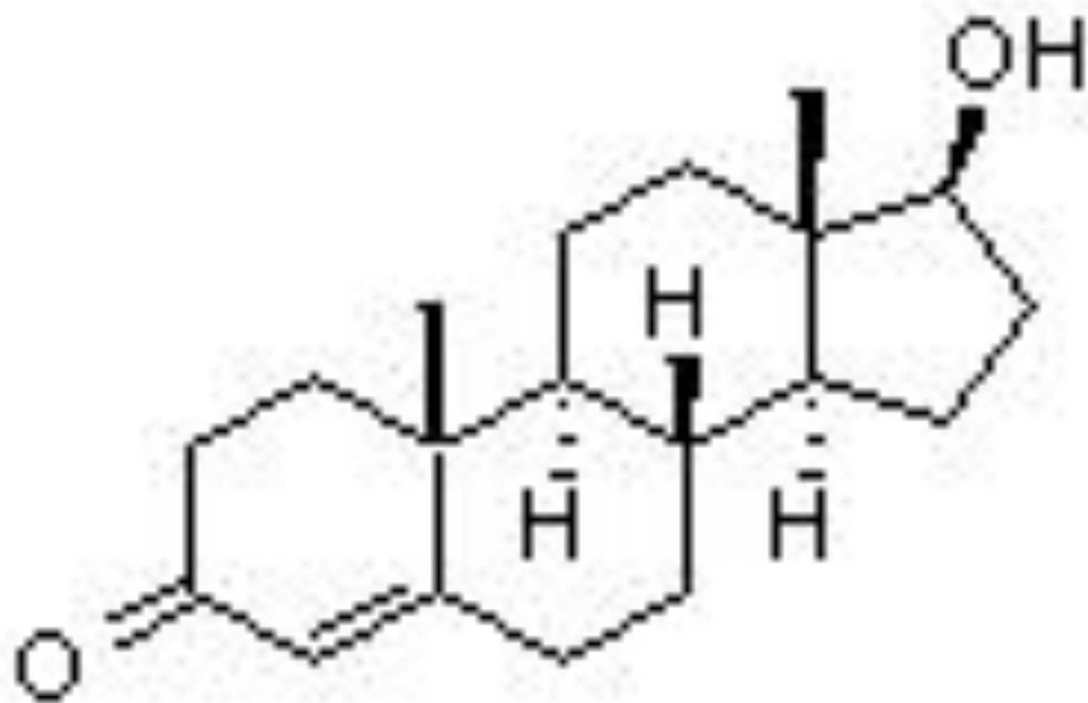
Testosterone
